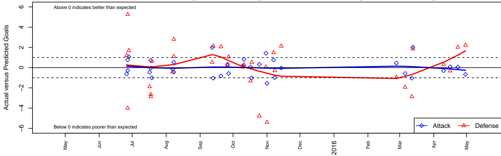
CSC Storm White G03 Dots are actual minus expected GF (blue circles) and GA (red triangles). Blue line is smoothed change in attack strength. Red is smoothed change in defense strength.
